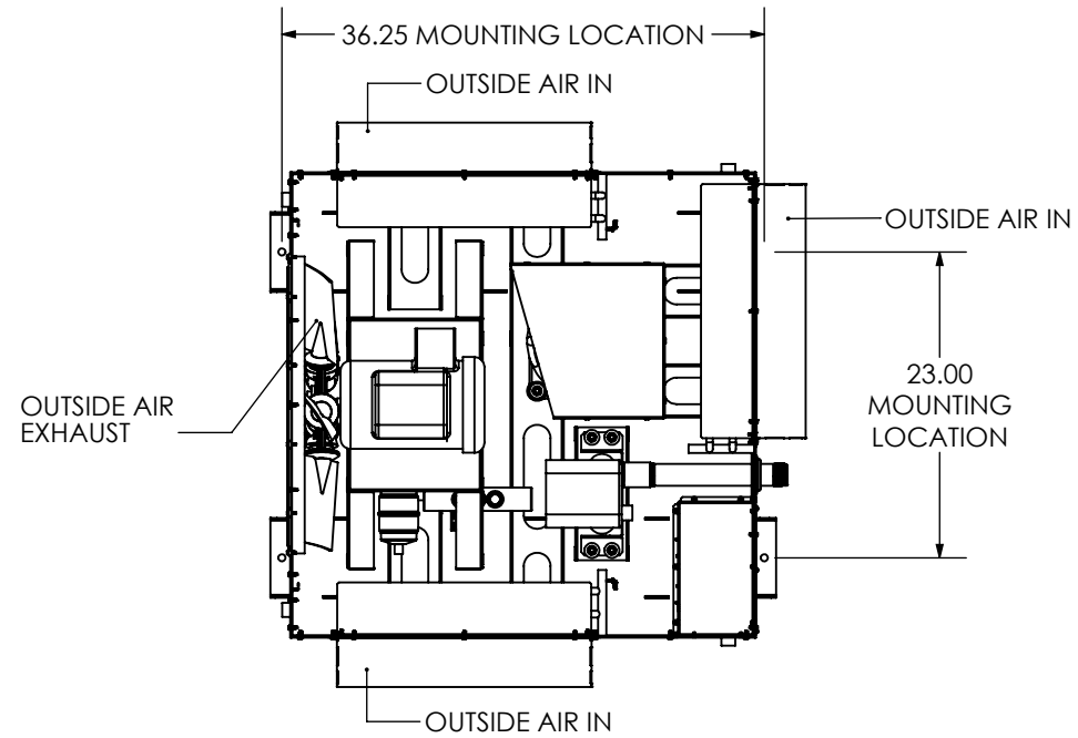
TOP VIEW WITH LID REMOVED FOR CLAIRITY
